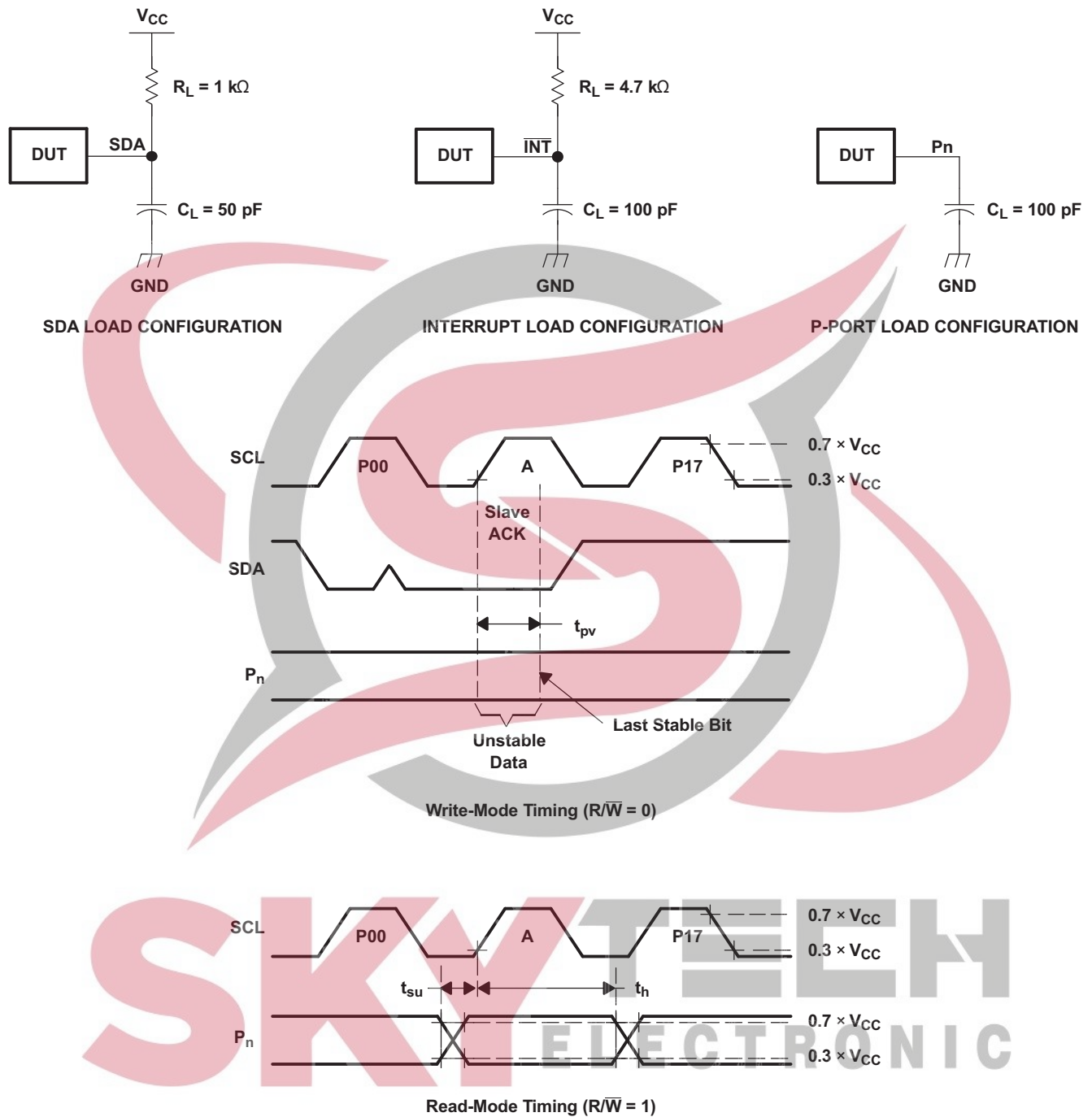
Figure 14. P-Port Load Circuits and Voltage Waveforms
